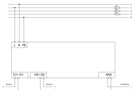
Exemplary circuit diagram SCN-DALI32.03
